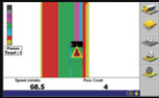
Operator view of pass count mapping
