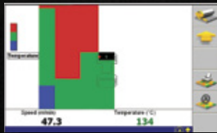
Operator view of temperature mapping
